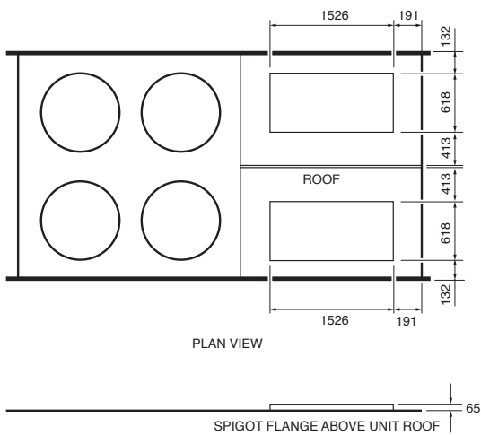
Upward Supply & Return Air versions
