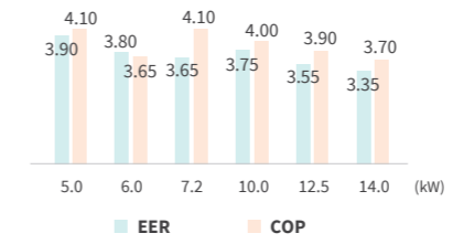
MSP Ducted unit
