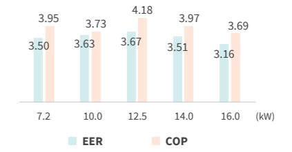
HSP Ducted unit
